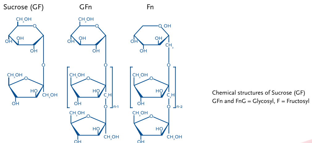
Fig. 4: The chemical structures in comparison.
